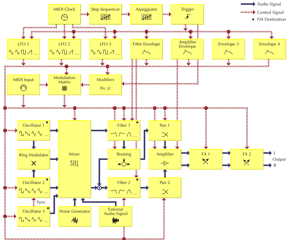
Picture 10: Block schematic diagram of a sound
