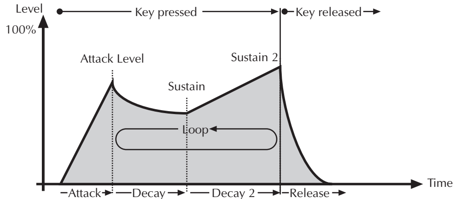
Picture 42: Loop S1S2 Envelope
